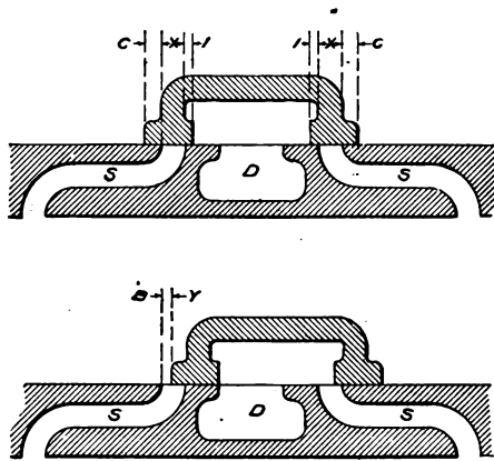
FIG. 327.—Diagrams illustrating the "Lap" and "Lead" of a Steam Cylinder Slide Valve. In both sections, S and S are the steam ports, and D the exhaust. The upper section illustrates the "laps" of a valve; the space between the lines C and X giving the "outside lap," and between the lines X and I the "inside lap." The lower section illustrates the "lead" of a valve; the space between lines B and Y showing the opening of the valve at the beginning of the right-hand stroke.
